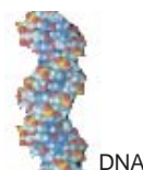
DNA
