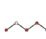
Molecule
