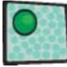
Plant cell
